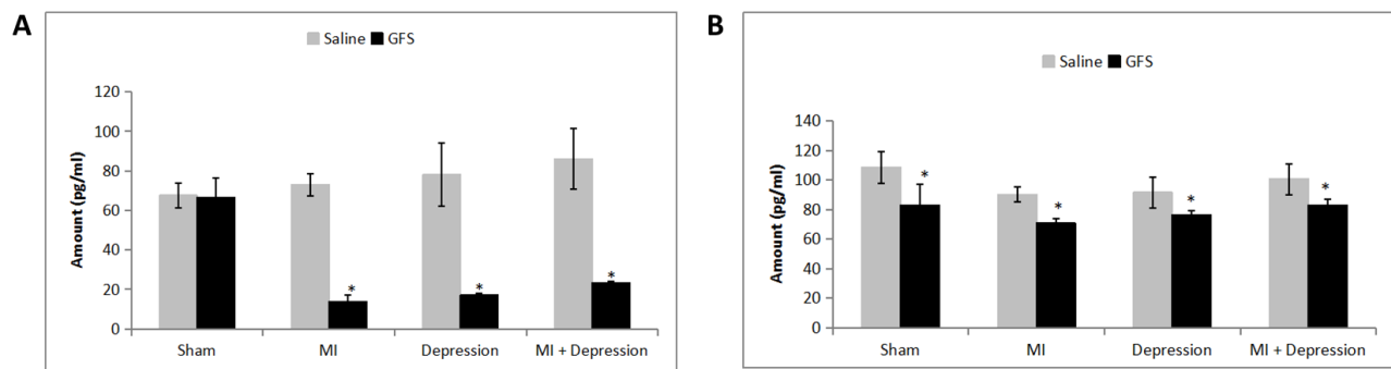
Figure 2. 5-HT 2A R levels were measured in the platelets and brain tissues using an ELISA kit. Data are presented as mean \pm SD. A) Platelet 5-HT 2A R quantification. There was no significant difference in 5-HT 2A R levels between the saline- and GFS-pretreated groups in the sham subgroup ( p=0.838 ). GFS pretreatment induced significant decreases in the MI, depression and MI + depression subgroups. * p<0.01 vs. saline, n=10 per subgroup. B) Brain 5-HT 2A R quantification. All four subgroups demonstrated significant decreases in 5-HT 2A R levels after GFS pretreatment. * p<0.01 vs. saline, n=10 per subgroup.
